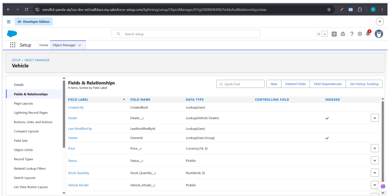
Figure 11: Fields and Relationships of the Vehicle object: Dealer lookup, Price, Status, Stock Quantity and Vehicle Model
